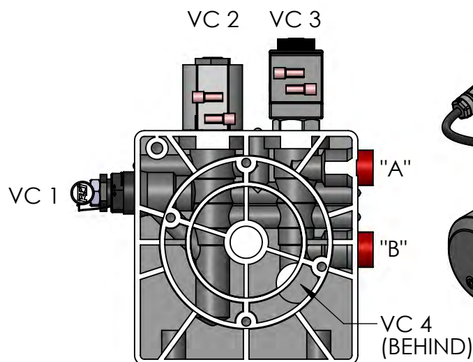
HYDRAULIC CIRCUIT 111
