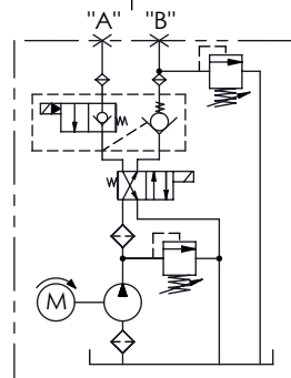
HYDRAULIC CIRCUIT 111
