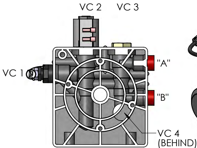
HYDRAULIC CIRCUIT 114
