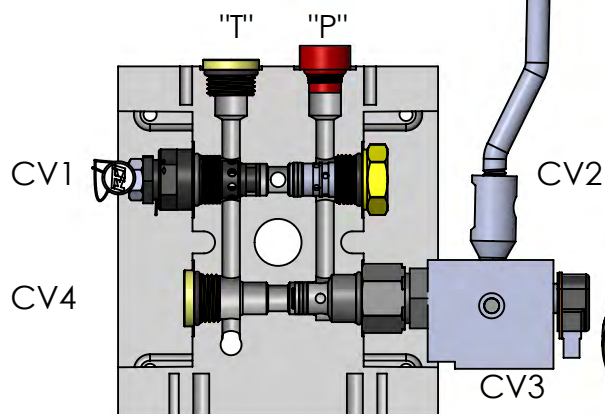
HYDRAULIC CIRCUIT 106
