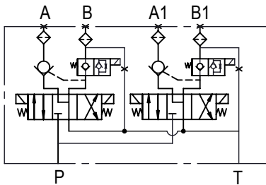
(2) 4w3p motor center cartridge solenoid valve (option: 4w3p close center cartridge valve) (2) KTI proprietary load holding valve
