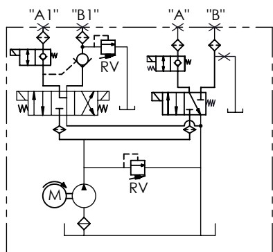
HYDRAULIC CIRCUIT 215
