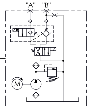
HYDRAULIC CIRCUIT 110
