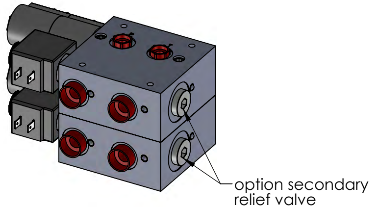
(2) 4w3p motor center cartridge solenoid valve (option: 4w3p close center cartridge valve) (2) KTI proprietary load holding valve
