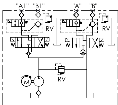
HYDRAULIC CIRCUIT 211
