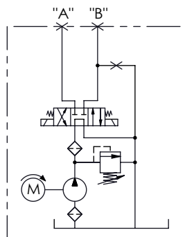
HYDRAULIC CIRCUIT 114B
