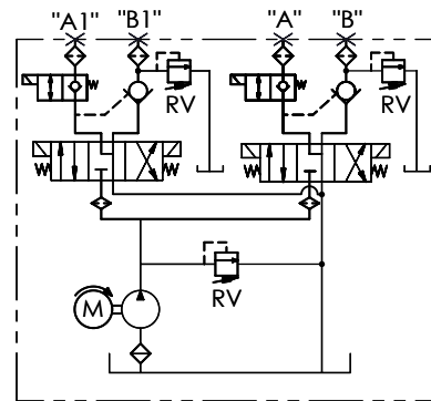
HYDRAULIC CIRCUIT 211
