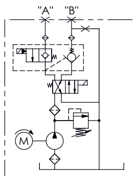
HYDRAULIC CIRCUIT 110
