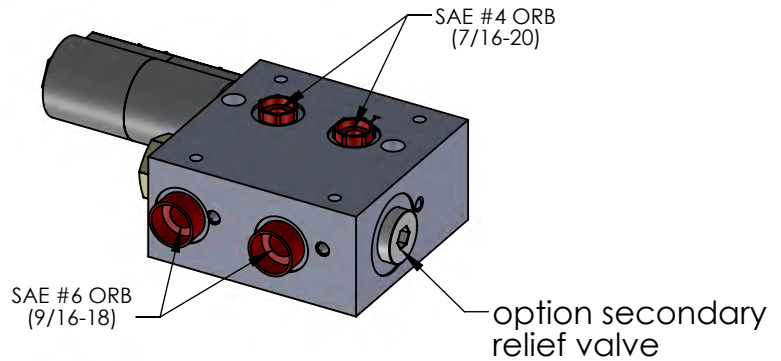
4w3p motor center cartridge solenoid valve (option: 4w3p close center cartridge valve) 4way cavity plug
