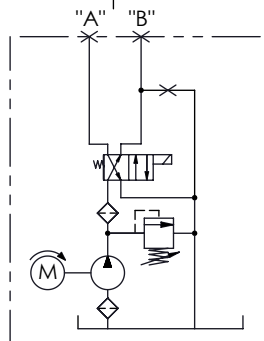
HYDRAULIC CIRCUIT 114
