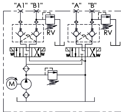
HYDRAULIC CIRCUIT 208
