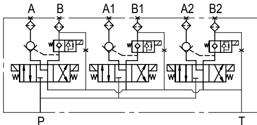
(3) 4w3p motor center cartridge solenoid valve (option: 4w3p close center cartridge valve) (3) KTI proprietary load holding valve
