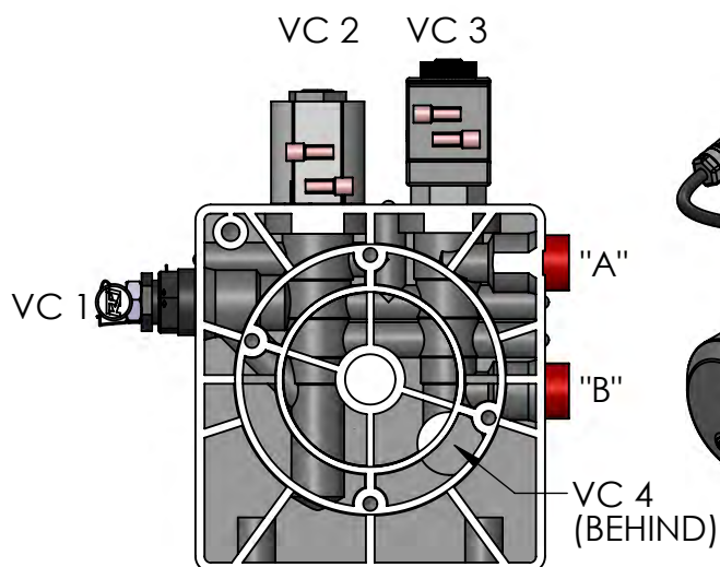
HYDRAULIC CIRCUIT 109
