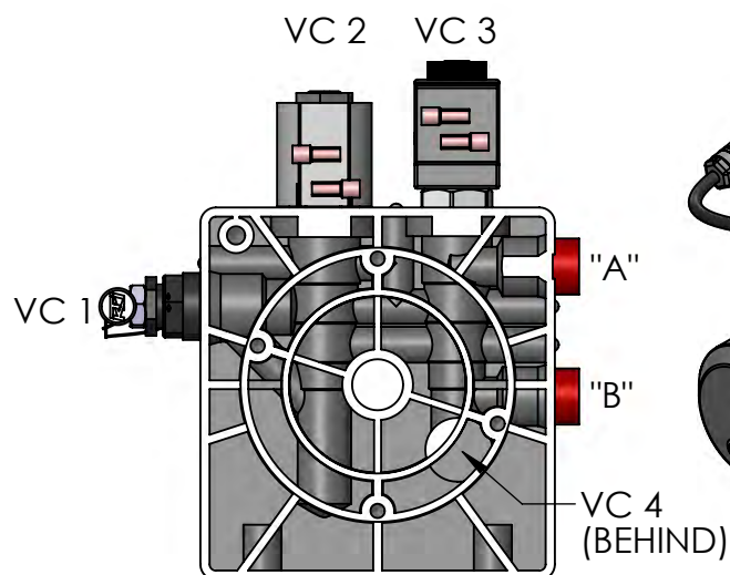
HYDRAULIC CIRCUIT 110
