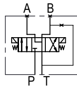
4w3p motor center cartridge solenoid valve (option: 4w3p close center cartridge valve) 4way cavity plug
